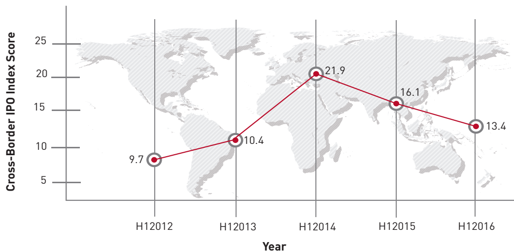
Cross-Border IPO Index Scores: H1 2012 - H1 2016
